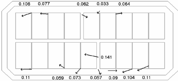
Figure 3: ALBRAS metal velocity measurements (m/s)
