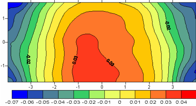
Figure 4: Metal-bath interface shape (m) obtained by the Shallow Layer model for the modified AP13 cell.
