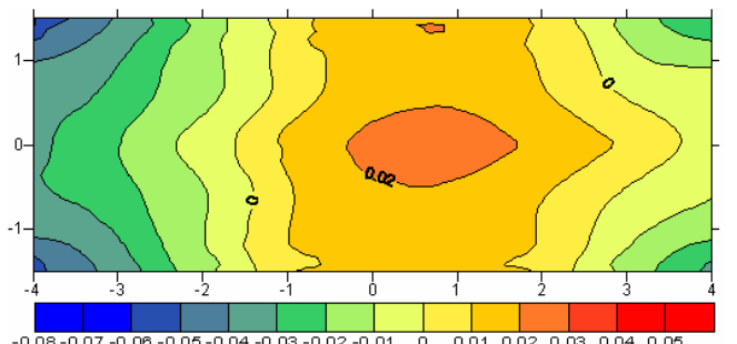
Figure 18: Metal-bath interface deformation (m) obtained by the Ansys CFX 3-phase model for the benchmark case
