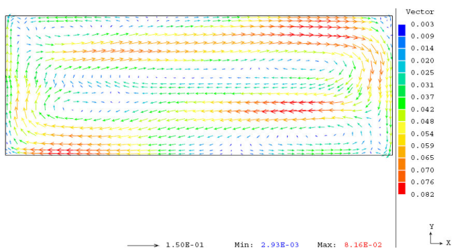
Figure 17: Metal flow (m/s) obtained by ESTER for the benchmark.
