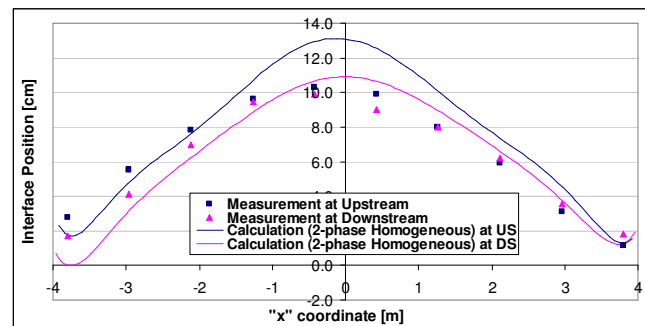
Figure 8: Metal-bath interface shape, calculated by CFX 2-phase Homogeneous model versus measured.
