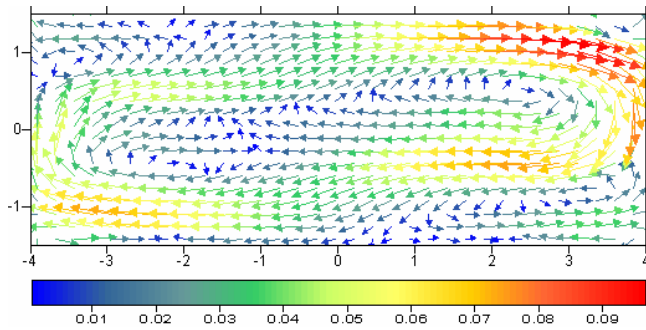
Figure 19: Metal flow (m/s) obtained by the Ansys CFX 3-phase model for the benchmark case
