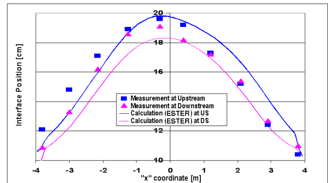
Figure 7: Metal-bath interface shape, calculated by ESTER model versus measured.
